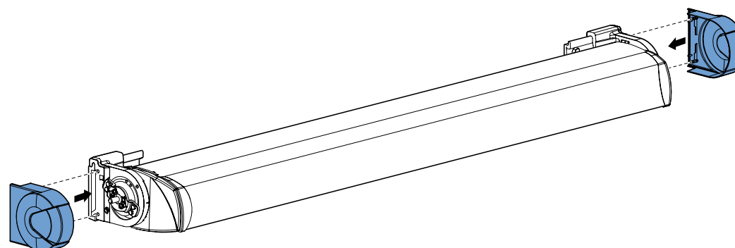
fig. 7.2 Mounting the plastic side covers (optional)
