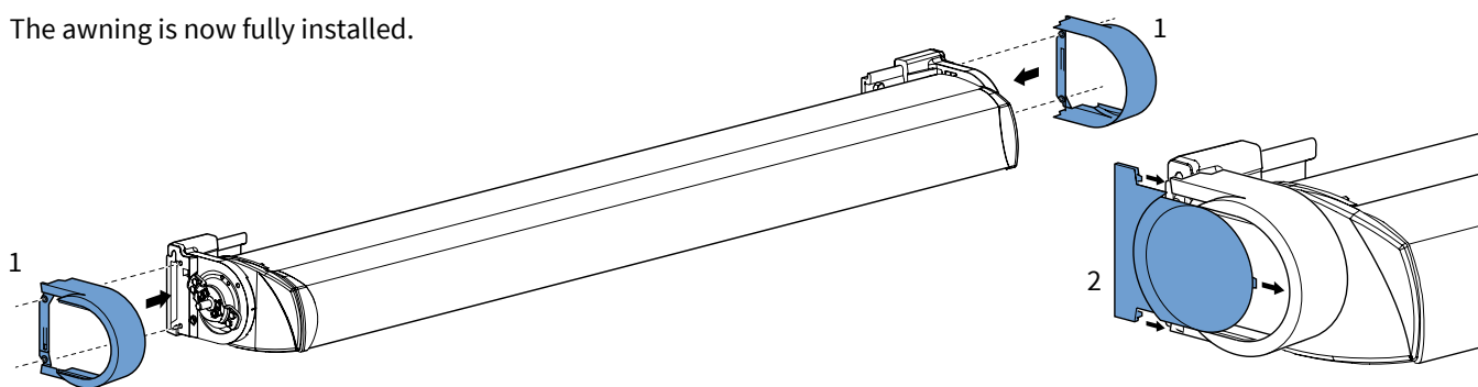
fig. 7.1 Mounting the aluminium side covers
