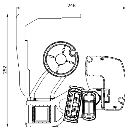
Awning section
