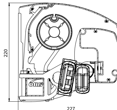
Awning section with cover (optional)
