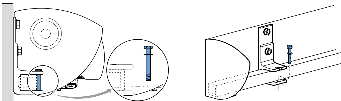
fig. 2.3 Applying locking bolt
