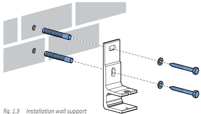
fig. 1.3 Installation wall support
