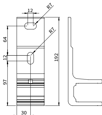
Front view wall support
