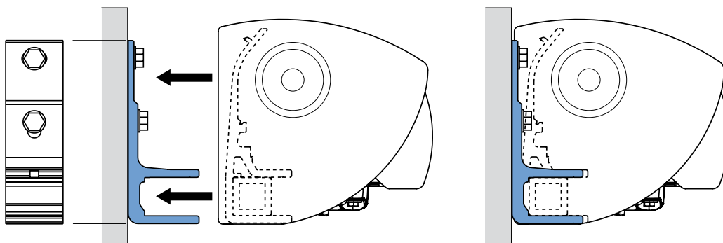
fig. 2.2 Detail wall support
