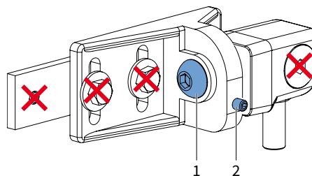
fig. 6.3 Detail arm-connection
