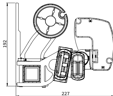
Awning section
