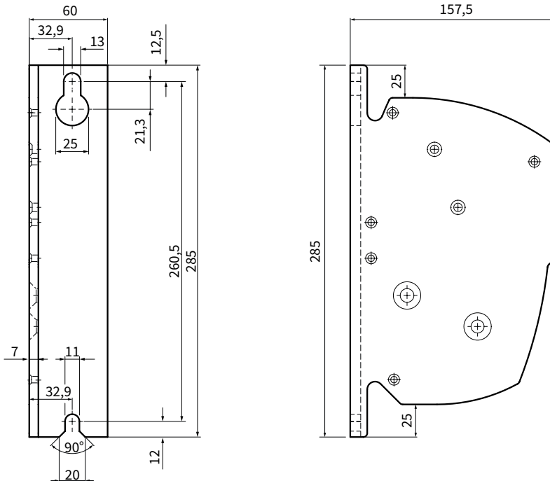
Front view left wall support
