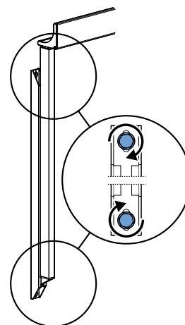
fig. 7.4 Fixing of the bolts
