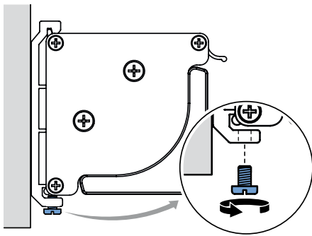
fig. 2.6 Applying the securing bolts
