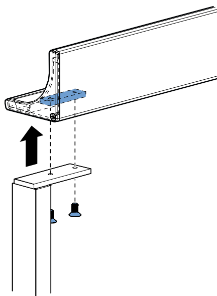
fig. 3.8 Fixating the drop-arm
