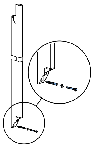
fig. 2.2 Fixate the bottom of the drop-arm
