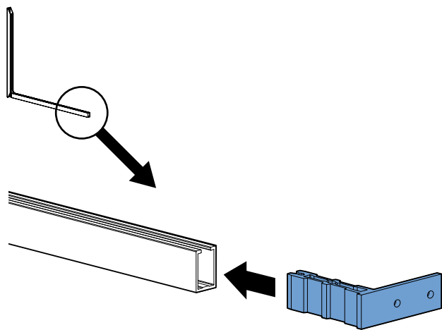
fig. 2.5 Sheet in the arms
