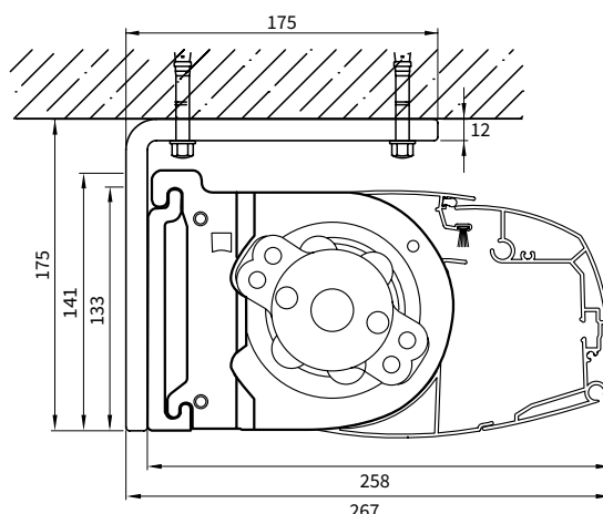
Awning section
