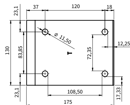
Top view ceiling support
