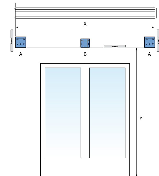
fig. 1.1 Placing wall supports
