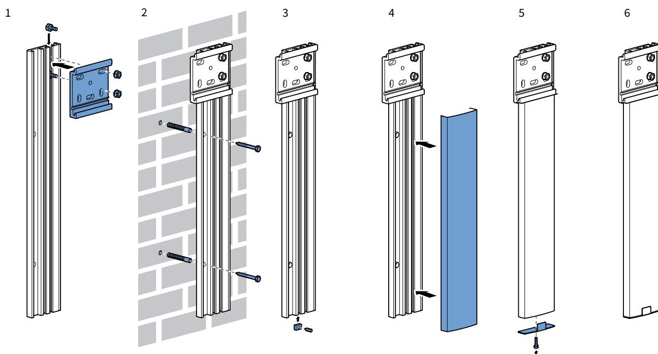
fig. 8.2 Mounting the wall strip right
