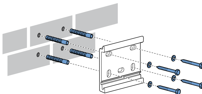
fig. 1.2 Mounting the wall supports
