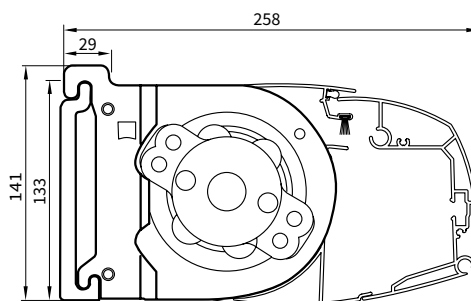
Awning section
