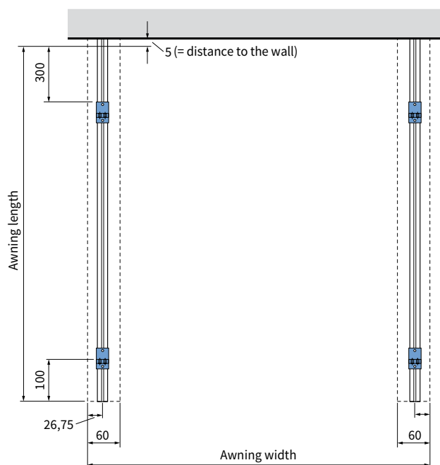
Fig. 5 Top view, mounting feet
