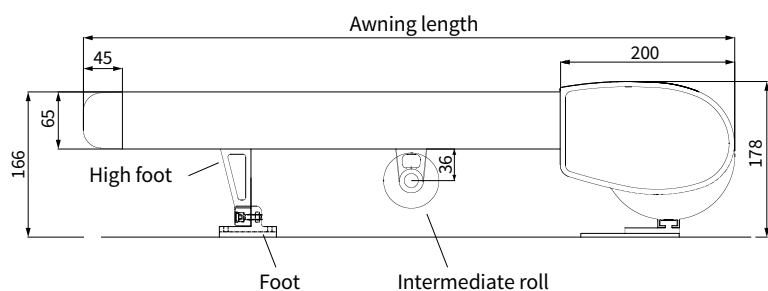
Fig. 1 Side view
