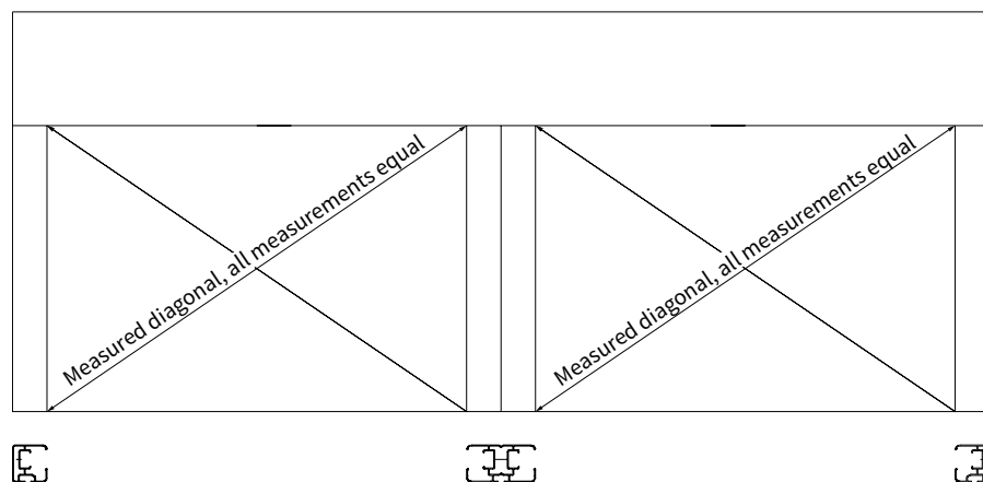
Fig. 6 Top view
