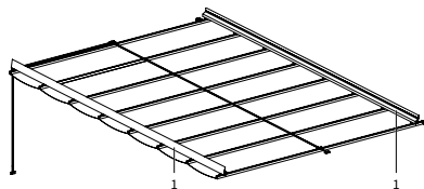
3 meters wide conservatory blind with side guides (1) installed on the outside
