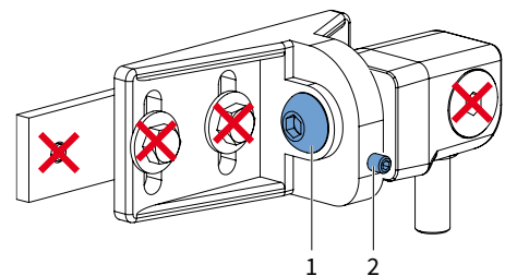
fig. 6.3 Detail armverbinding
