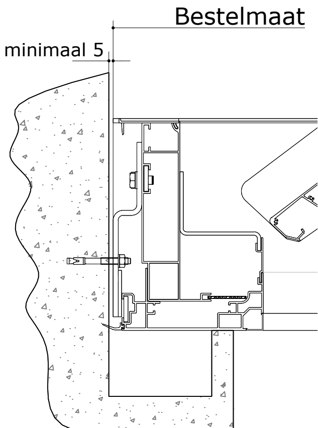
V870 - Arezzo - 017.dwg
