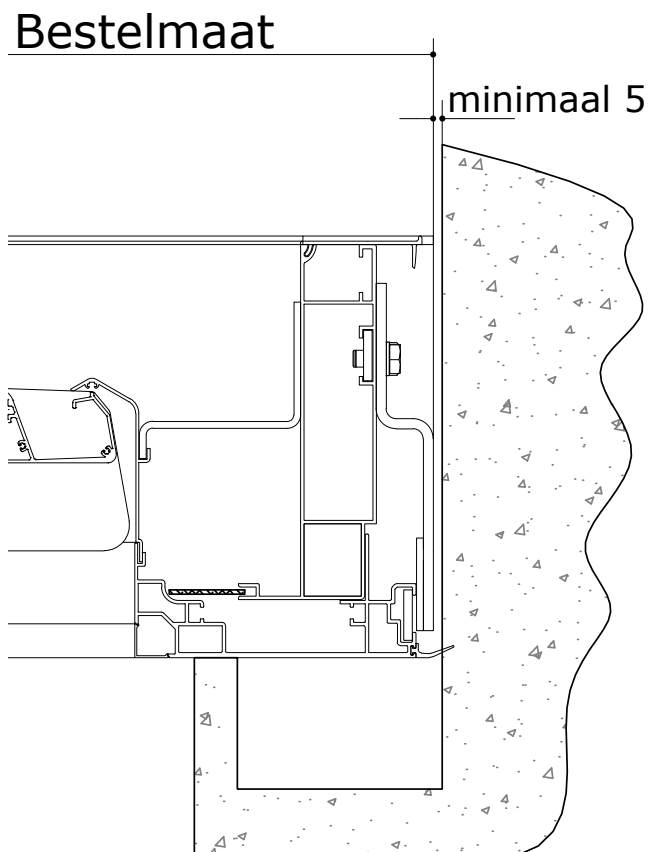
V870 - Arezzo - 018.dwg
